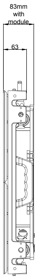
Right view
